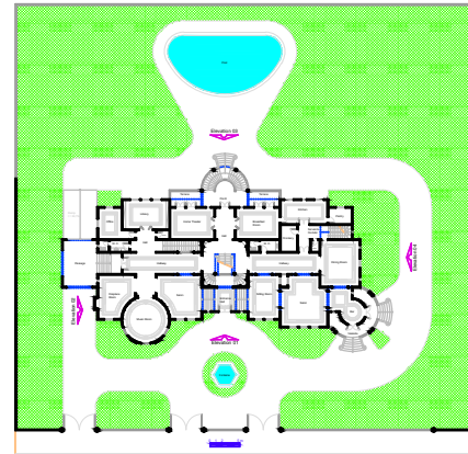
First Floor Plan A = 596,79 m 2
